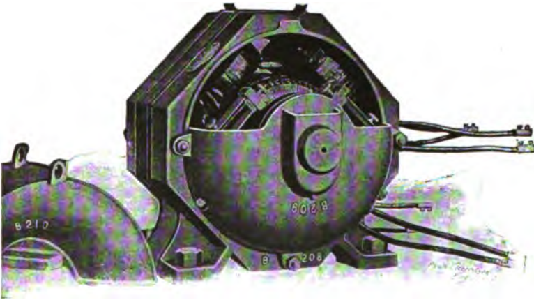
FIG. 432.—The "Lundell" Octagon Motor, with case open, showing parts.
